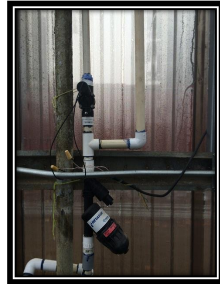
Filter, regulator and auto valve for mist.
